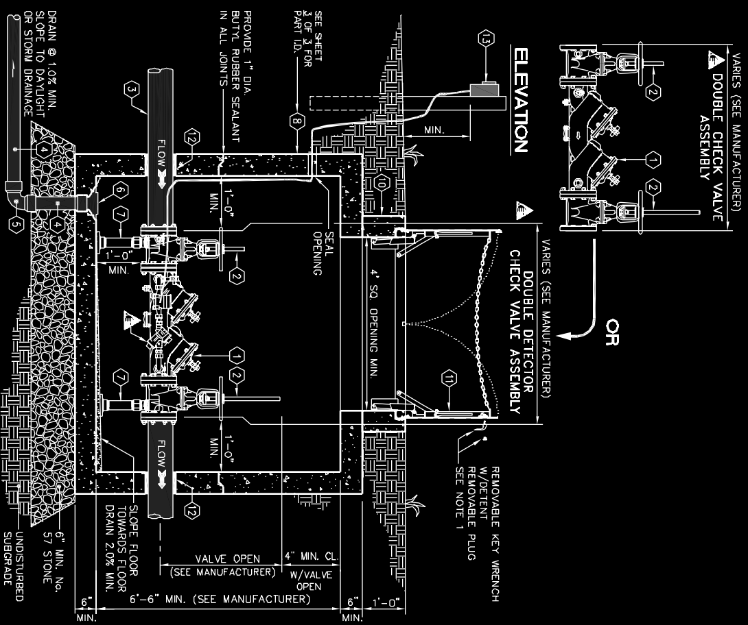
2 1/2" to 10" DCV, DDCV ASSEMBLY (UNDER GROUND VAULT)
